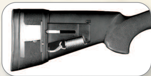
HORIZONTAL VARIABLE RATIO CAM RECOIL SYSTEM
